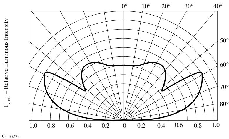
95 10275 Figure 4. Rel. Luminous Intensity vs. Angular Displacement
