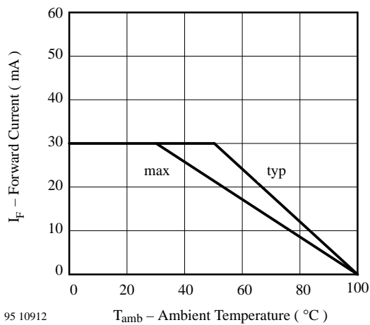
95 10912 Figure 2. Forward Current vs. Ambient Temperature
