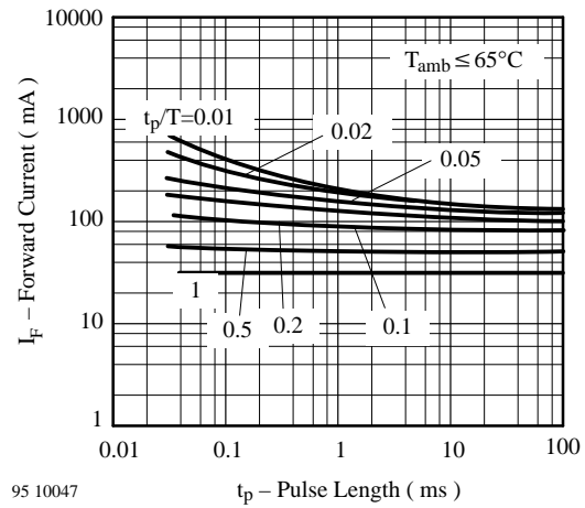
95 10047 Figure 3. Forward Current vs. Pulse Length
