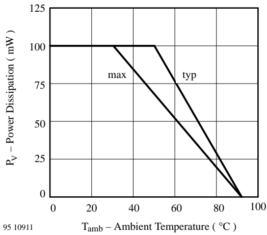
95 10911 Figure 1. Power Dissipation vs. Ambient Temperature
